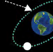
MOON PROXIMITY
