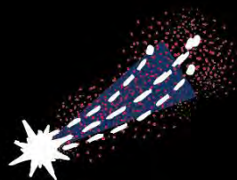
METEOR SHOWERS
