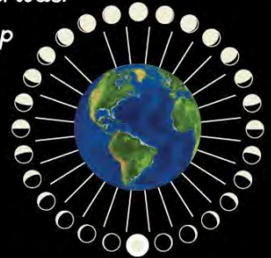
MOON PHASES
